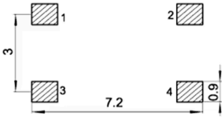
PBC Layout
